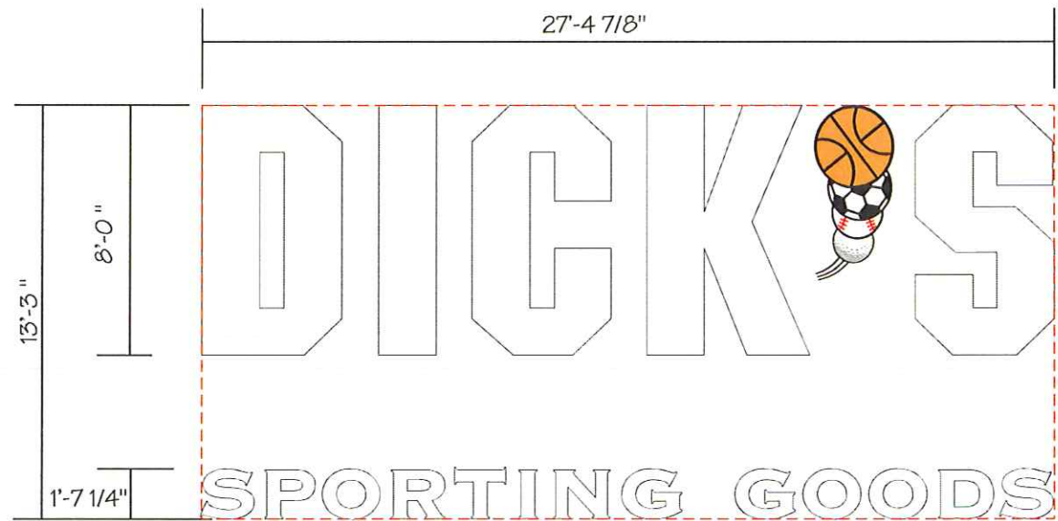
Internally Illuminated Channel Letters Scale: 3/16" = 1'
