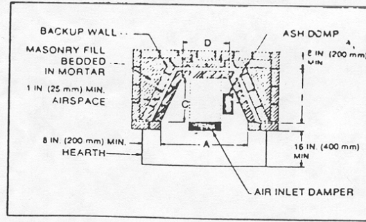
Single-Face Fireplace Plan FIG. 1b
