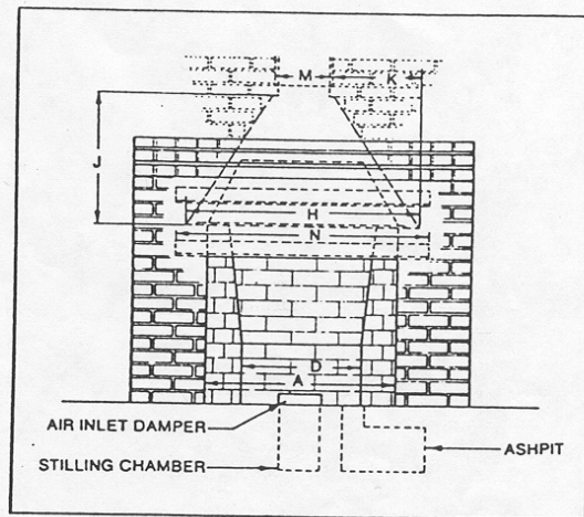
Single-Face Fireplace Front Elevation FIG. 1c
