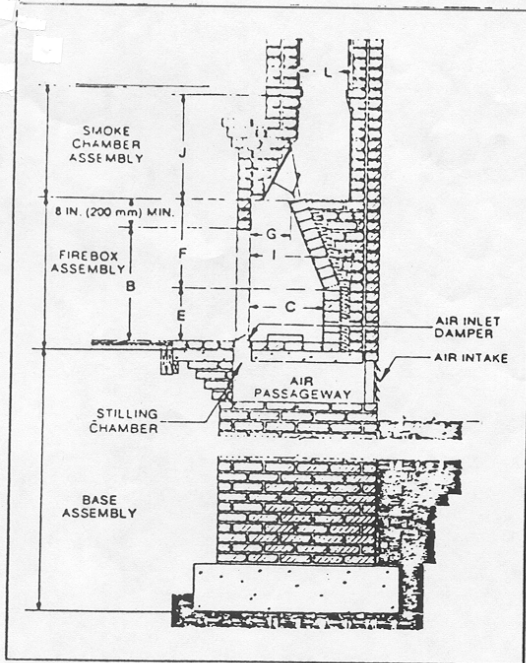
Single-Face Fireplace Section FIG. 1a
